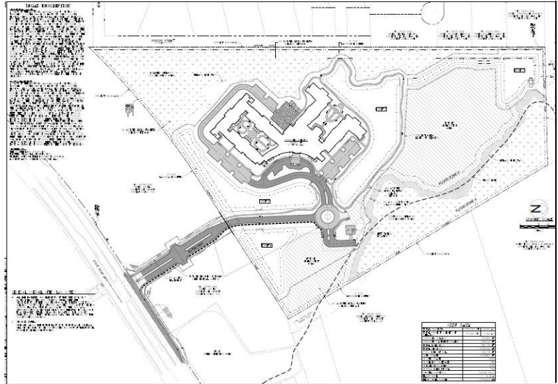
Site plan for Silver Creek Assisted Living Facility located on SR 207 near St. Augustine
